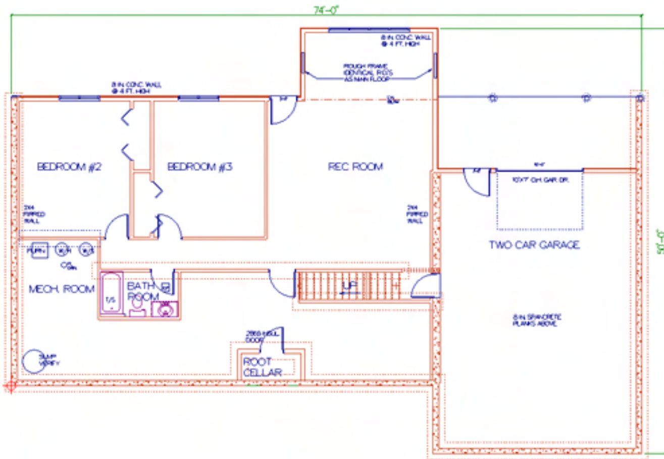
BASEMENT PLAN
